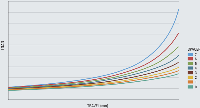
EXAMPLE SPRING CHARACTERISITIC: DUROLUX EQ 29, 160mm travel
