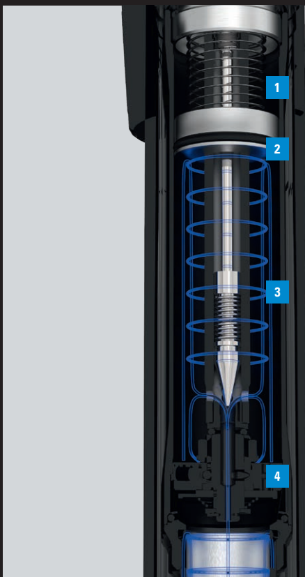
LOW SPEED COMPRESSION
