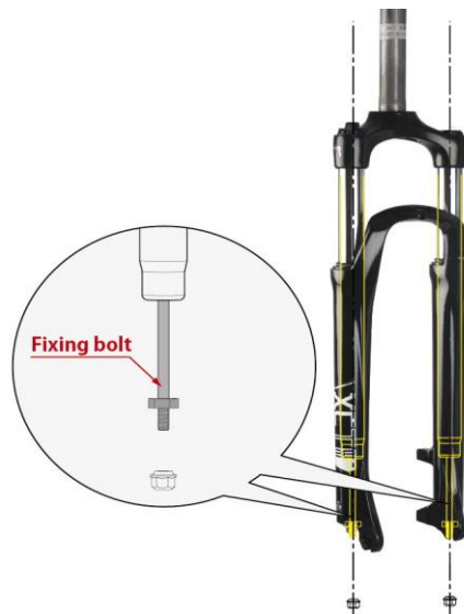
Figure: Multiple fixing bolt version
