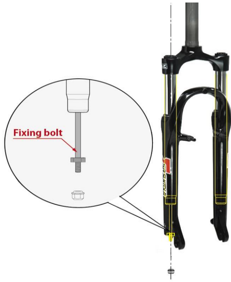
Figure: Multiple fixing bolt version 單邊固定螺絲版本(right side only 只有右側)
